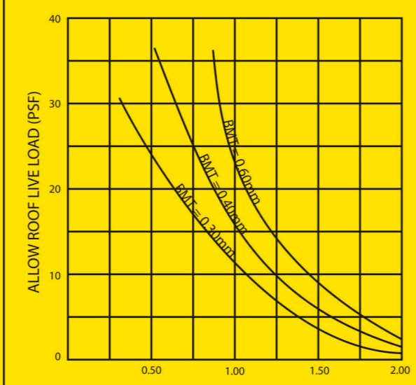
LOADING CHART FOR RIBSTAR HP LONGSPAN @ 1/240 DEFLECTION CONTINUOUS OVER TWO SPANS.
